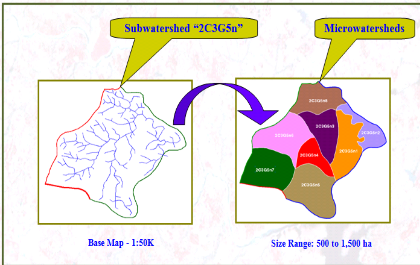
Fig. 7: Delineation of Microwatersheds from Subwatershed
